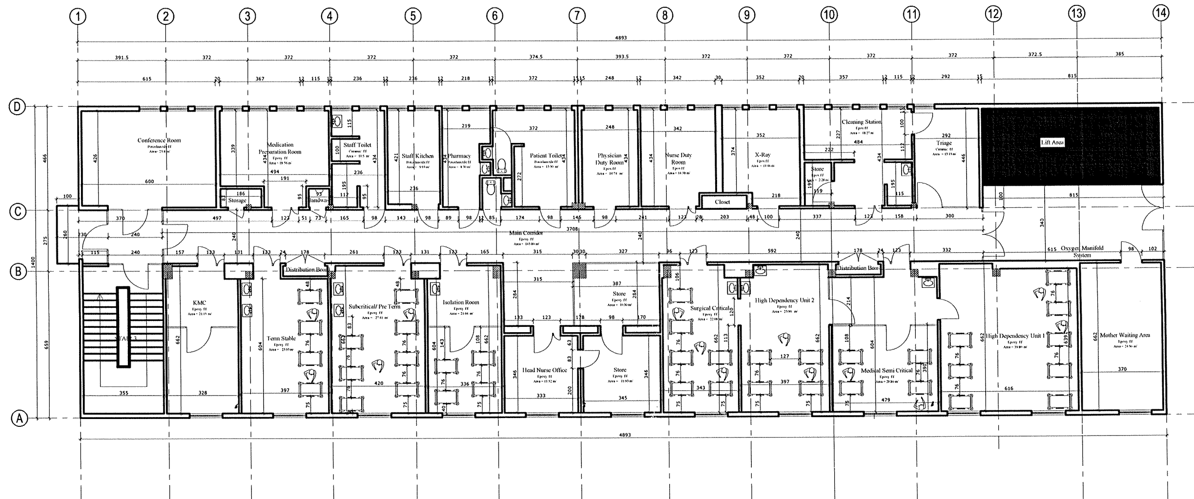
NICU Floor Plan Scale 1:80
